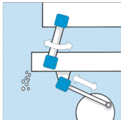
Shaker conveyor
